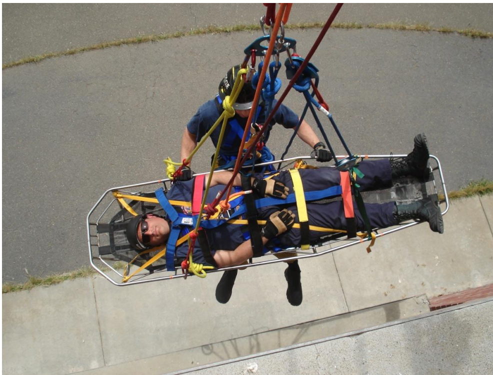
Figure 15-14. The patient is secured into the litter but still connected to their own system.
