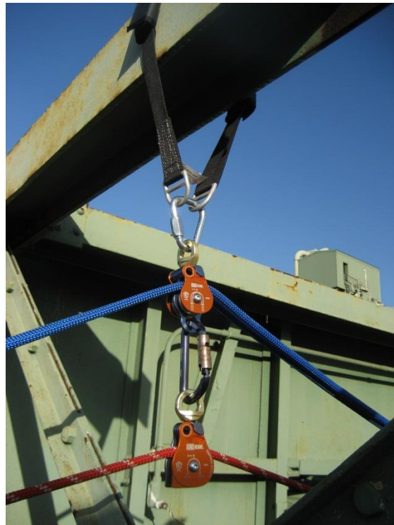
Figure 17-2. A Structural High Directional
