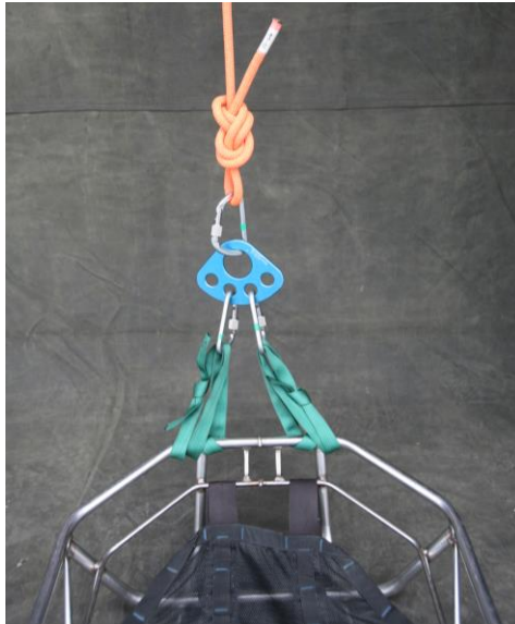
Figure 15-2. Litter rigged for a vertical lower/raise. Second line omitted for picture clarity.
