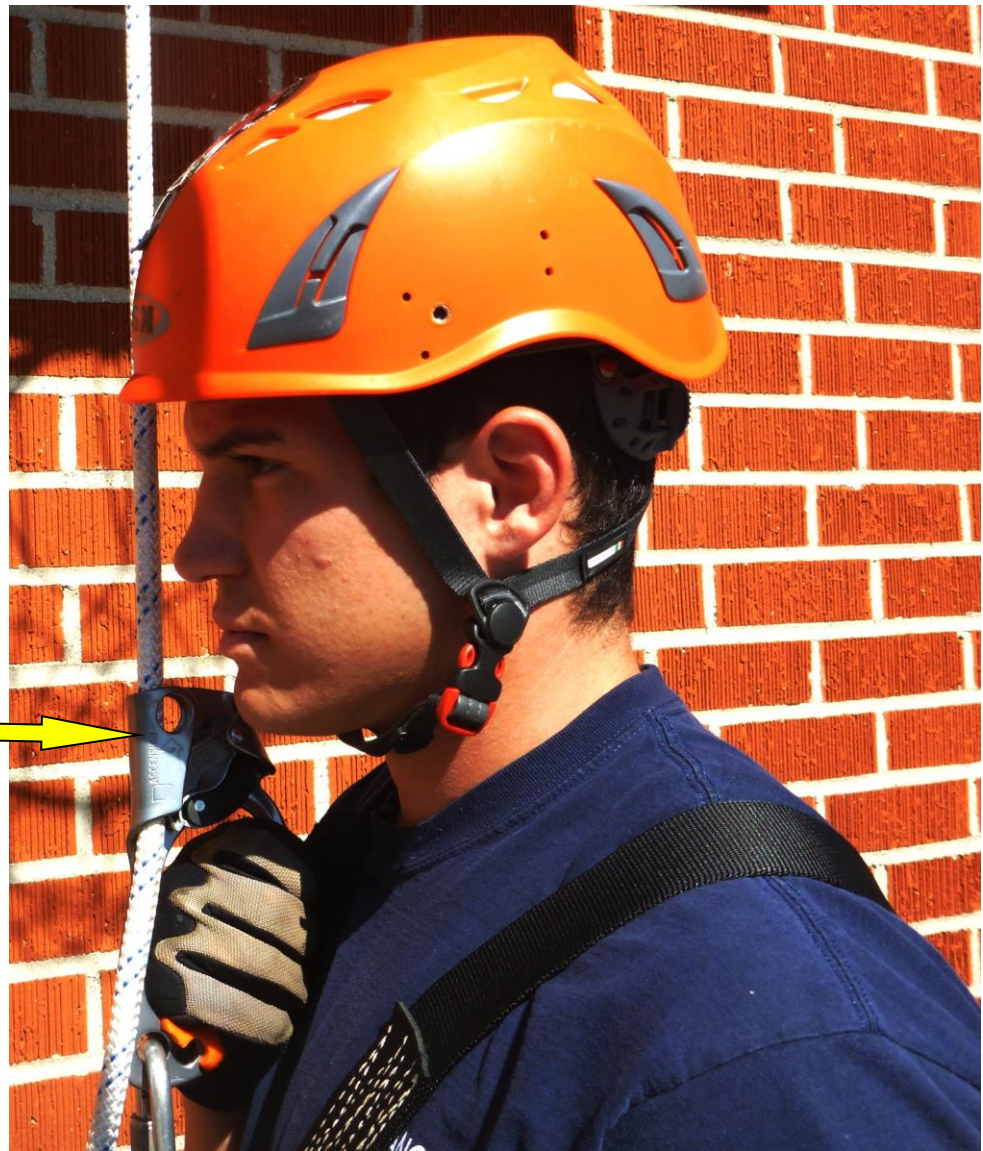
Figure 12-6. Adjusting Lead ascender
