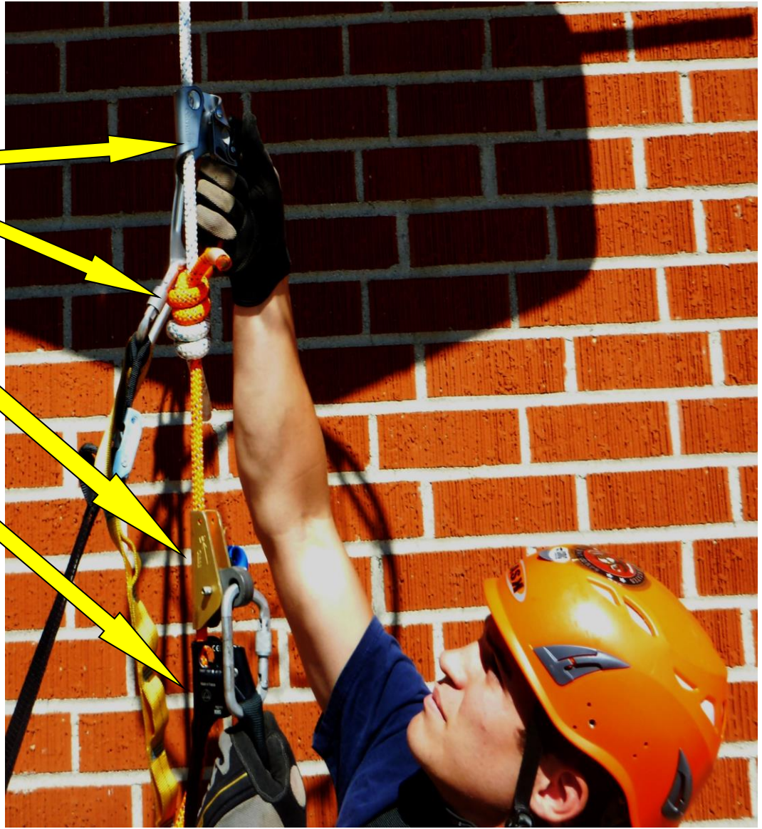
Figure 12-11. Reattaching lead ascender above the knot
