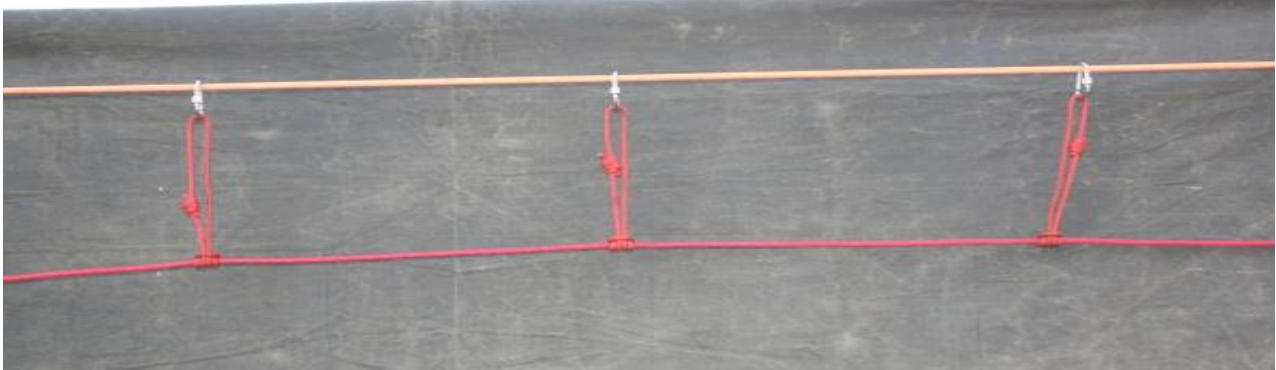
Figure 17-1. Tagline Hangers
