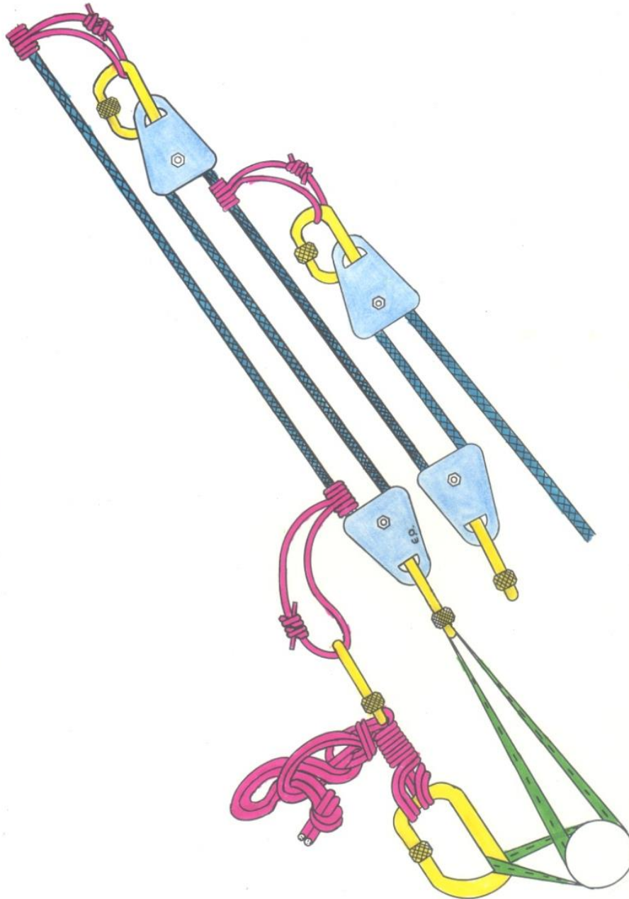
Figure 8-4. 9:1 Compound Mechanical advantage (3:1 X 3:1 = 9:1)
