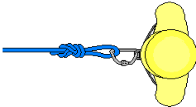
Figure 6-2. Non-adjustable attachment at the rescuer.
