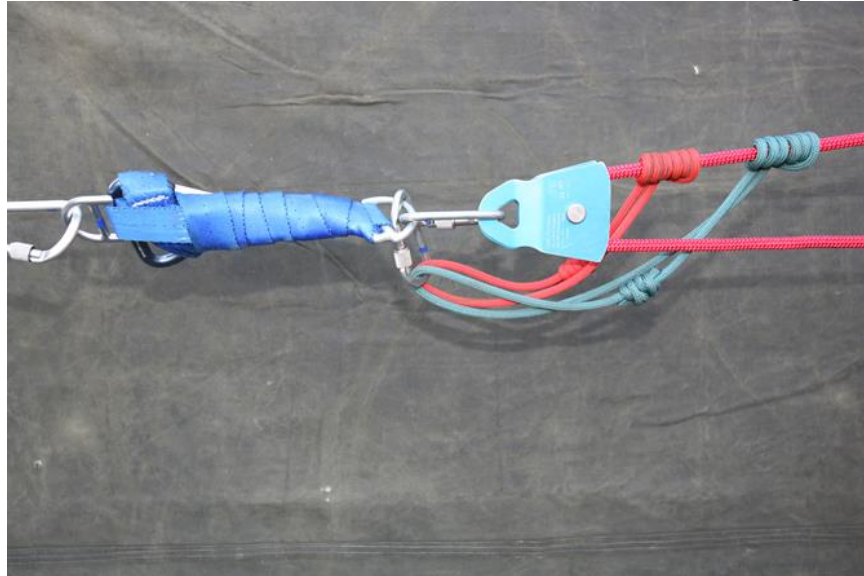
Figure 17-5. Tagline with Tandem Prusiks
