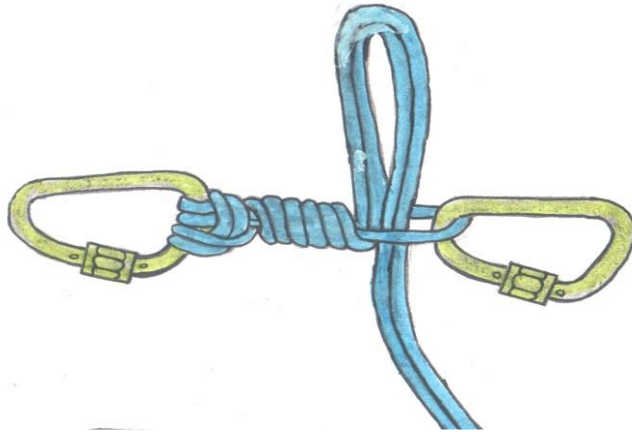
FIGURE 9-7. Step 2 Untying.
